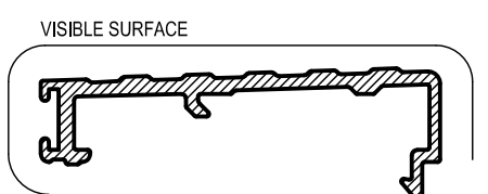
TSD165 RAMP THRESHOLD Mass. 0.4 Kg/m Anod. Per. 172 Paint Per. 100
