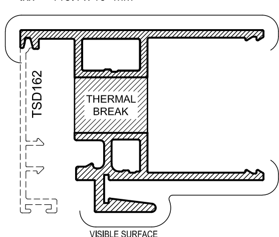
Mass. 1.403 Kg/m Anod. Per. 410 Paint Per. 175 Ixx = 115.1 x 10 3 mm 4
