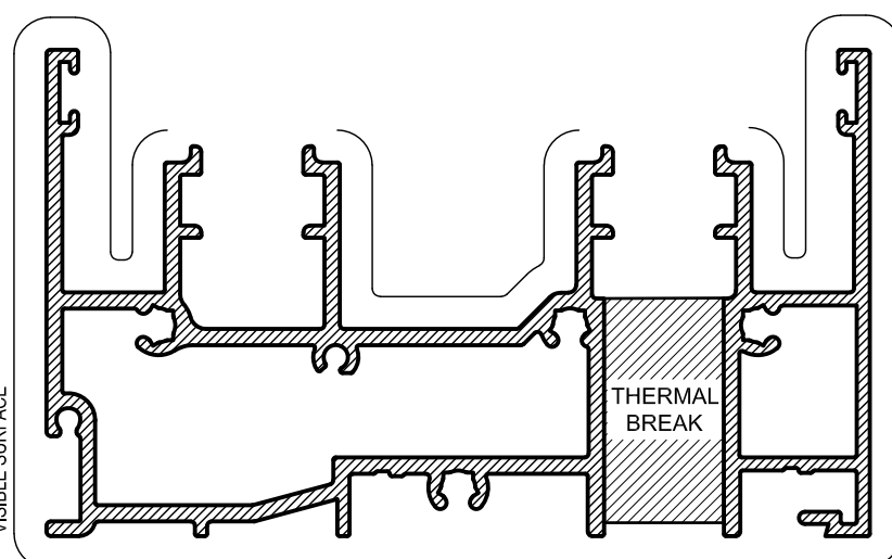
TSD243S 101.6mm SUMP SILL Mass. 2.668 Kg/m Anod. Per. 785 Paint Per. 340
