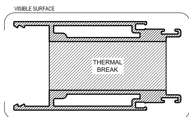
Mass. 1.552 Kg/m Anod. Per. 456 Paint Per. 166 Ixx = 105.7 x 10 3 mm 4
