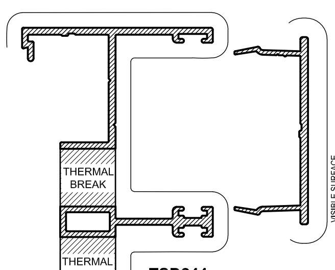
TSD244 101.6mm JAMB Mass. 1.602 Kg/m Anod. Per. 666 Paint Per. 292 Ixx = 564.8 x 10 3 mm 4
